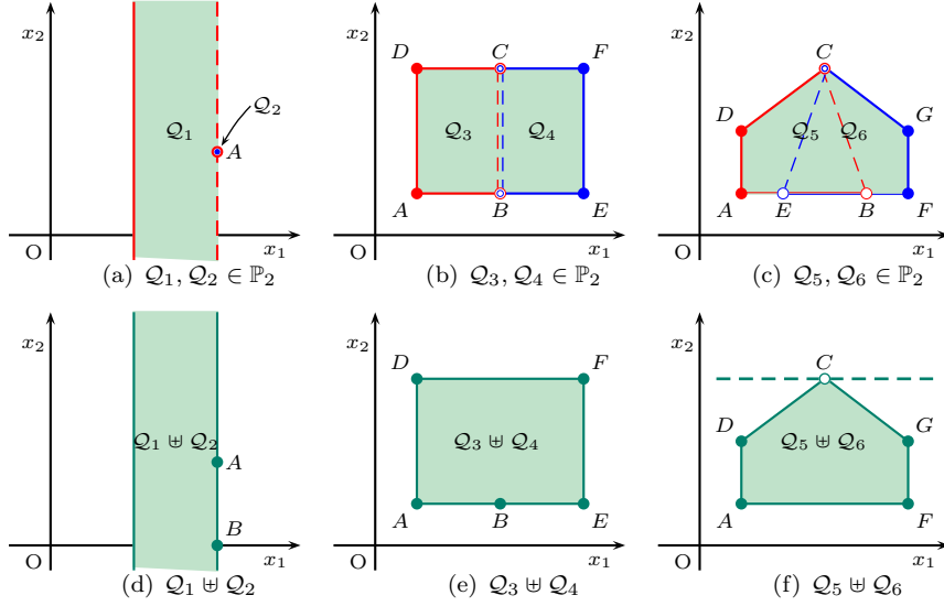
Figure 2: More examples for the convex polyhedral hull of NNC polyhedra
