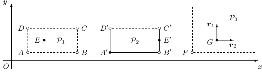
Fig. 1. Using closure points to define NNC polyhedra.
