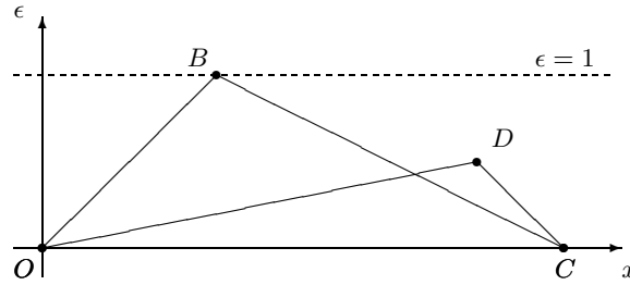
Fig. 5. Other two different \epsilon -representations for \mathcal{P}_3 , which can be obtained by applying the strong minimization process to the generator system describing \mathcal{R}_3 .
