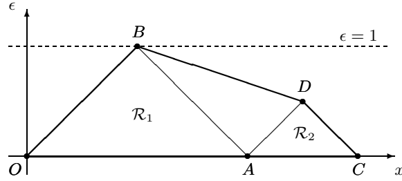
Fig. 2. The \epsilon -representations of \mathcal{P}_1 and \mathcal{P}_2 and of their poly-hull.
