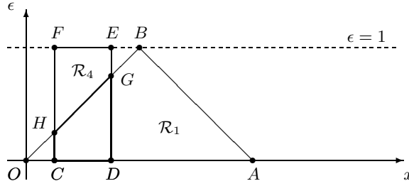
Fig. 3. The “minimized” trapezium CDGH , obtained by intersecting \mathcal{R}_1 and \mathcal{R}_4 and still representing the topologically closed NNC polyhedron \mathcal{P}_4 , also encodes the strict inequality x > 0 .
