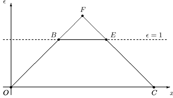
Fig. 4. The trapezium OCEB is obtained by applying the strong minimization process to the constraint system describing \mathcal{R}_3 . The triangle OCF is yet another representation for the NNC polyhedron \mathcal{P}_3 , which can be characterized by a constraint system and a generator system that are both in smf.
