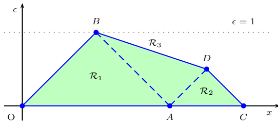
Fig. 4. The \epsilon -representations of \mathcal{P}_1 and \mathcal{P}_2 and of their poly-hull.
