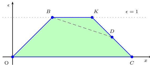
Fig. 6. The trapezium OCKB is an \epsilon -representations for \mathcal{P}_3 , obtained by applying the \epsilon -minimization process to the constraint system describing \mathcal{R}_3 .
