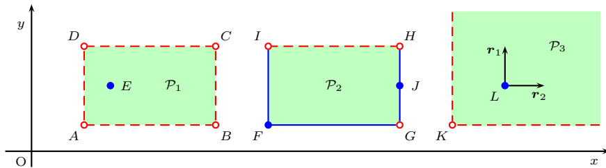
Fig. 1. Using closure points to define NNC polyhedra on \mathbb{R}^2 .
