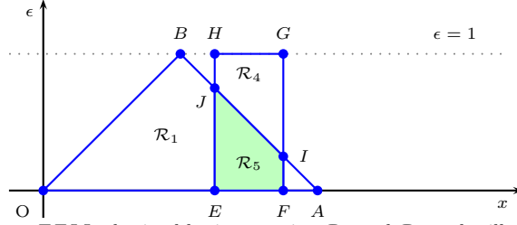
Fig. 5. The “minimized” trapezium EFIJ , obtained by intersecting \mathcal{R}_1 and \mathcal{R}_4 and still representing the topologically closed NNC polyhedron \mathcal{P}_4 , also encodes the strict inequality x > 0 .
