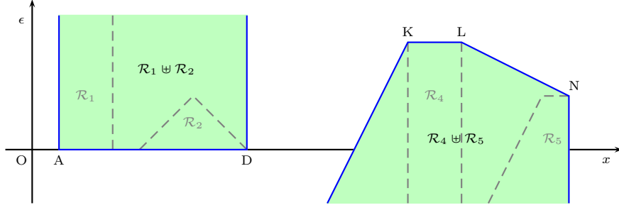
Fig. 3. \mathcal{R}_1 \uplus \mathcal{R}_2 (resp., \mathcal{R}_4 \uplus \mathcal{R}_5 ) does not represent the NNC polyhedron \mathcal{P}_1 \uplus \mathcal{P}_2 (resp., \mathcal{P}_4 \uplus \mathcal{P}_5 ).
